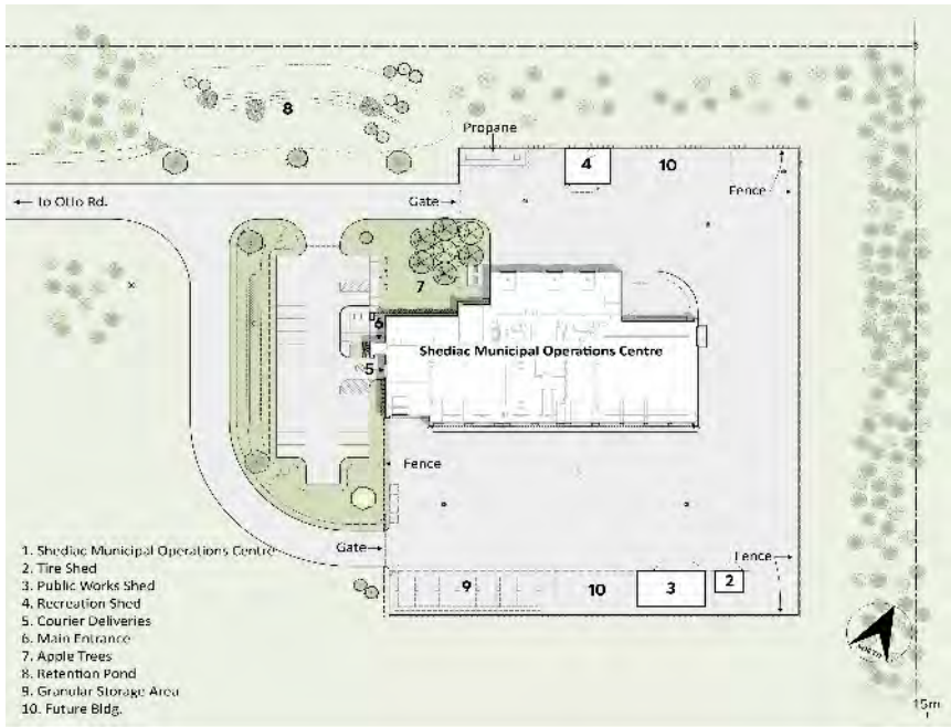
SITE PLAN
